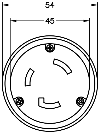
NEMA L5-30 CONNECTOR FRONT VIEW
